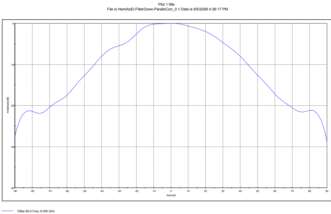
Figure 6b. IsoFilter TM ed Azimuth Cut of Horn Mounted Near the Edge of a 36 inch Diameter Ground Plane
