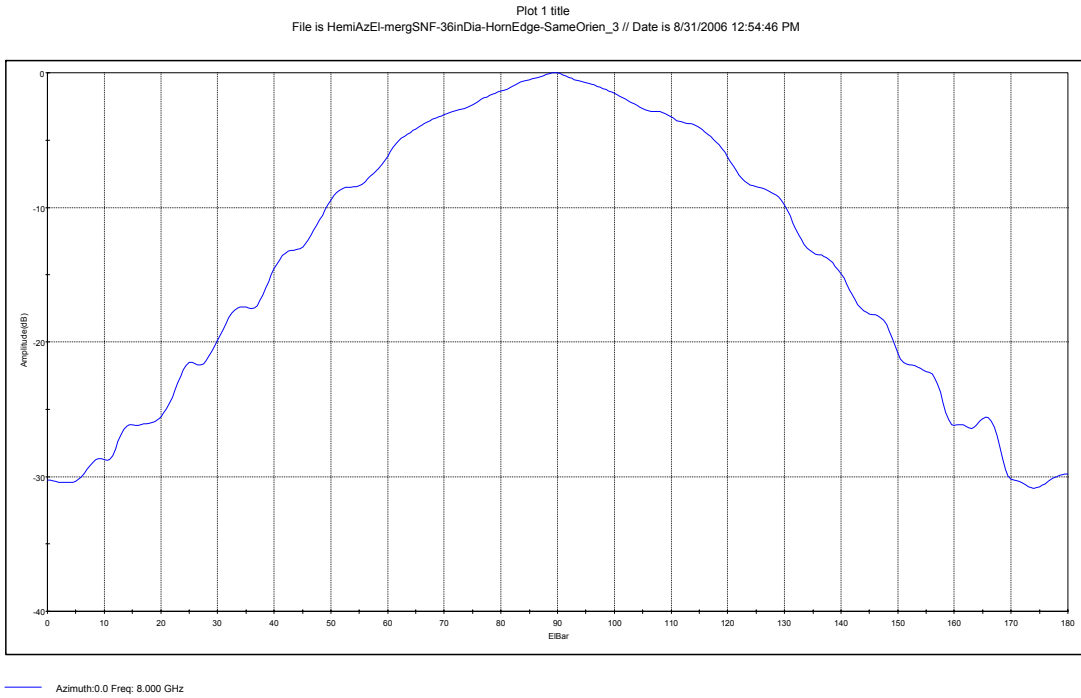
Figure 5a. Elevation Cut of Horn Mounted Near the Edge of a 36 inch Diameter Ground Plane
