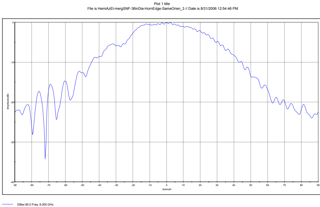
Figure 5b. Azimuth Cut of Horn Mounted Near the Edge of a 36 inch Diameter Ground Plane
