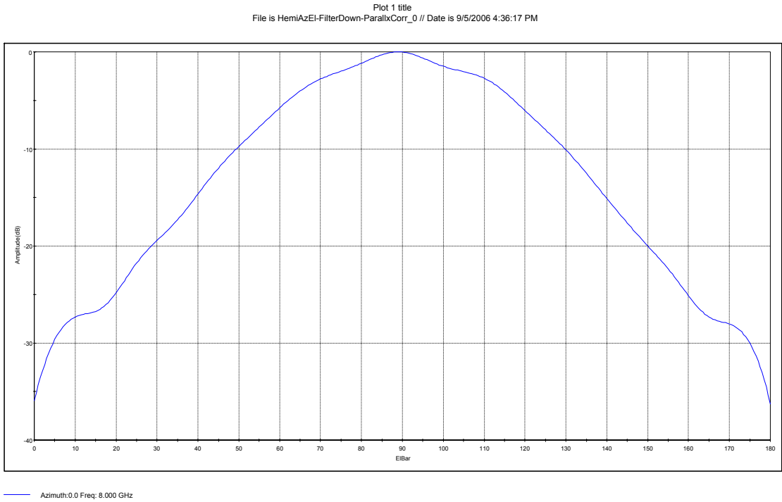
Figure 6a. IsoFilter TM ed Elevation Cut of Horn Mounted Near the Edge of a 36 inch Diameter Ground Plane
