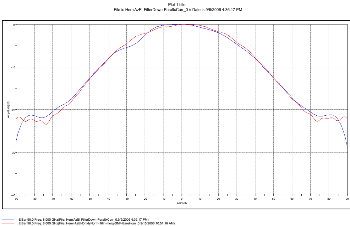
Figure 9b. IsoFilter™ 'ed Azimuth Cut of Horn Mounted Near the Edge of a 36 inch Diameter Ground Plane versus Centered Horn Mounted with Absorber Covering the Ground Plane.
