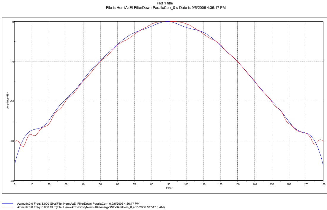
Figure 9a. IsoFilter™ 'ed Elevation Cut of Horn Mounted Near the Edge of a 36 inch Diameter Ground Plane versus Centered Horn Mounted with Absorber Covering the Ground Plane.
