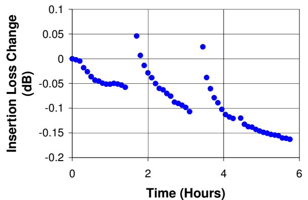
Figure 4 – Change in Cable's Insertion Loss During Six-Hour Test
