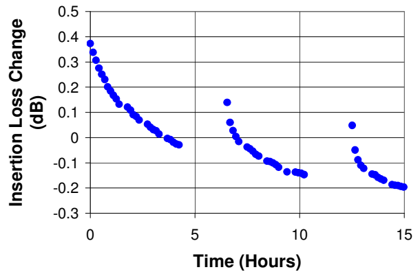
Figure 6 – Change in Cable's Insertion Loss During 15-Hour Test
