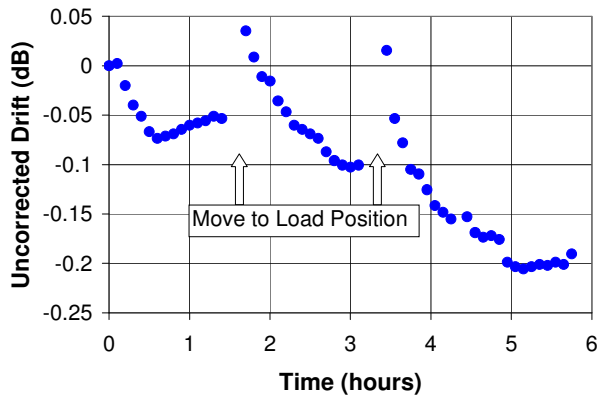
Figure 2 – Drift in Six-Hour Measurement
