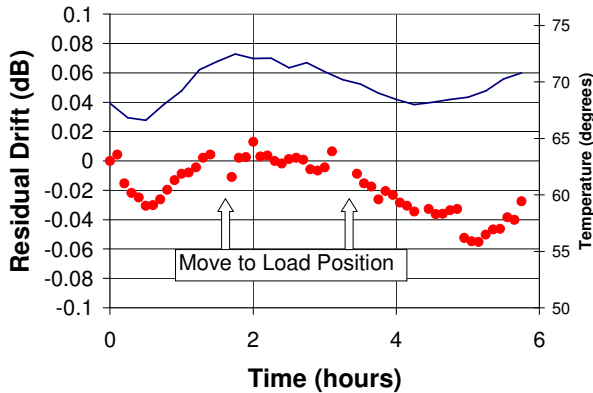
Figure 5 – Residual Drift for Six-Hour Test
