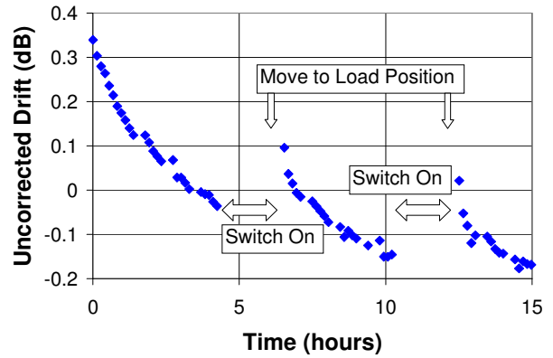
Figure 3 – Drift in 15-Hour Measurement
