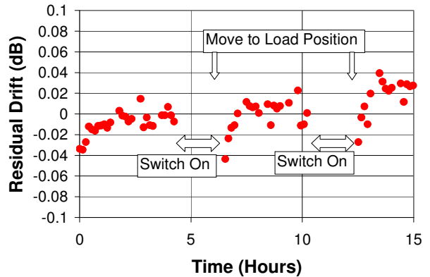
Figure 7 – Residual Drift for 15-Hour Test
