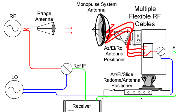
Figure 1 – Conceptual Cabling Diagram
