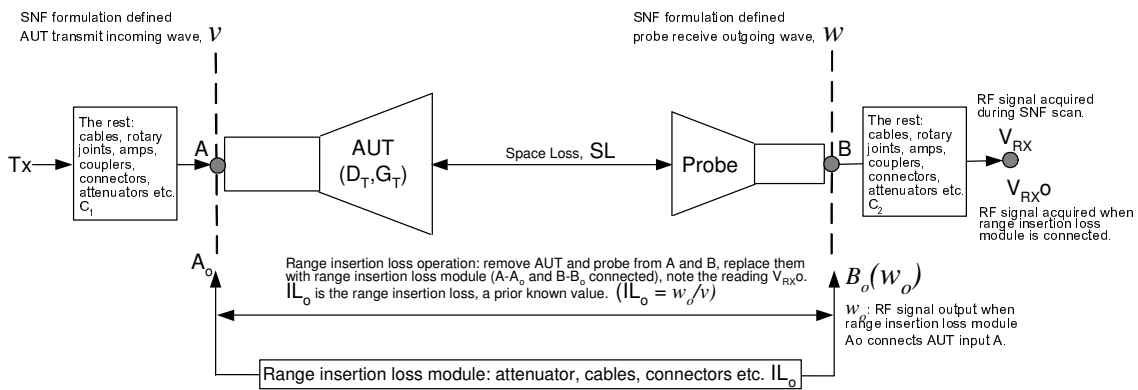
Figure 1 Illustrate parameters involved in SNF antenna measurement and range insertion loss measurement
