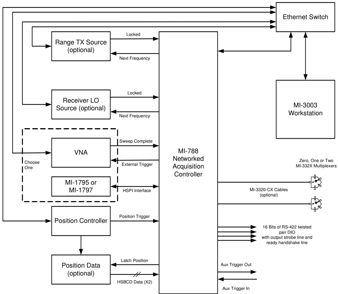
Figure 3 The MI-788 in a System
