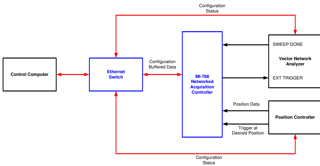
Figure 5 The Simple VNA based System with an MI-788 Included
