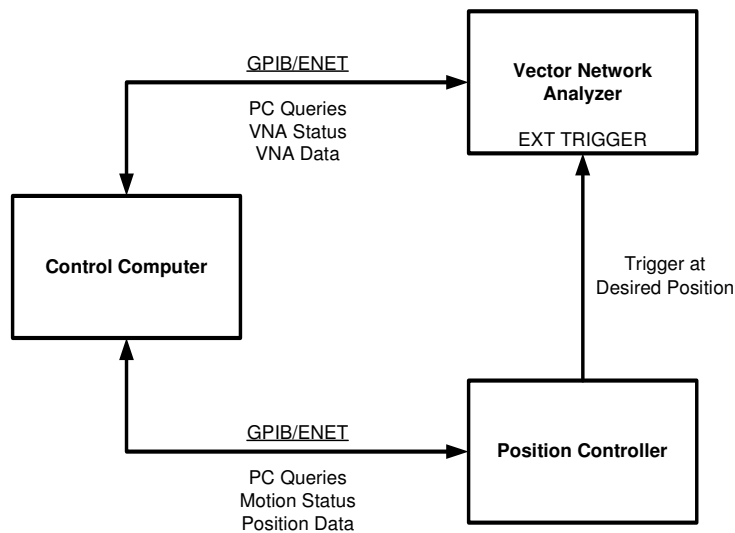
Figure 1 Simple VNA Based Measurement System
