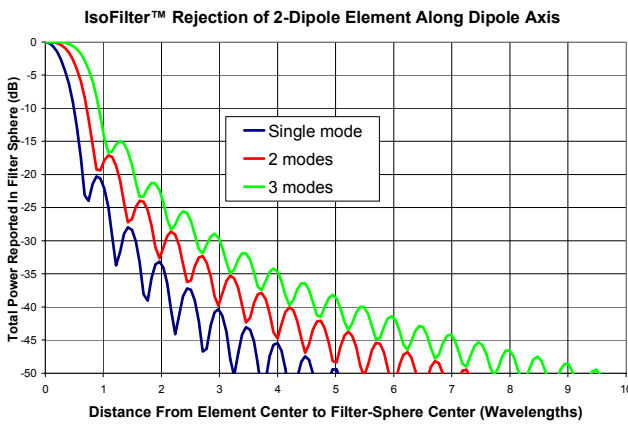
Figure 9 - Rejection Curve for Two-Dipole Element IsoFilter TM with Origin Translated Along x-Axis
