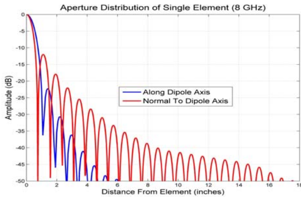
Figure 17 - Plot of Image Level versus Distance for Single Element at 8.0 GHz
