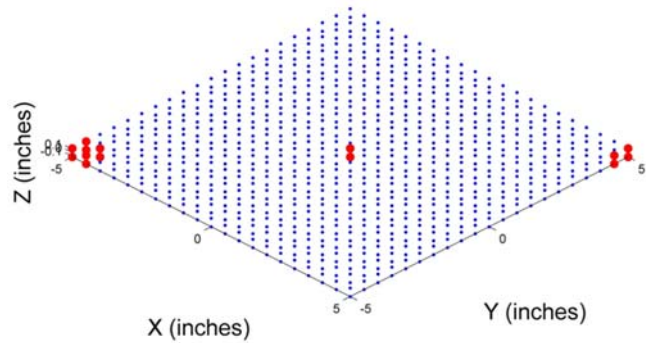
Figure 11 - Schematic of 21 X 21 Element Sparse Array
