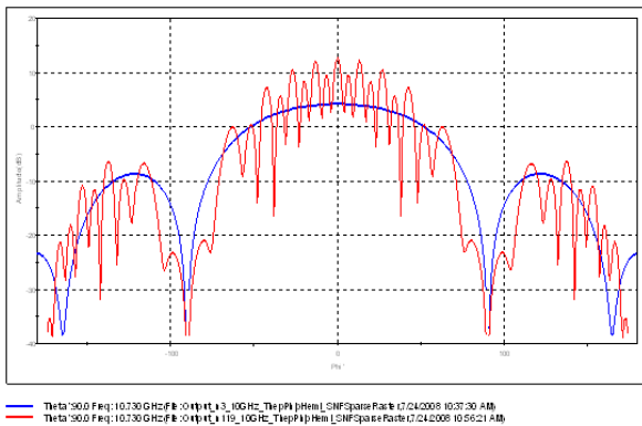
Figure 14 –Far Field of Sparse Array Before & After IsoFilter TM to Center Element
