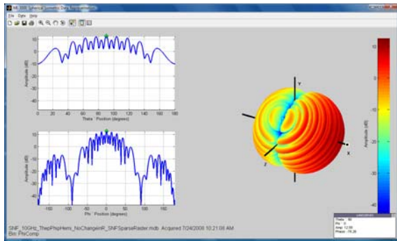
Figure 12 - Sparse Array's Far Field at 10.73 GHz.
