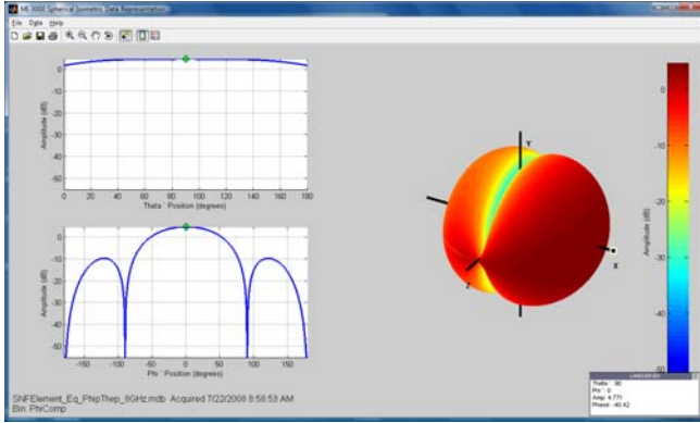
Figure 8 - Two-Dipole Element Pattern ( \phi Component)
