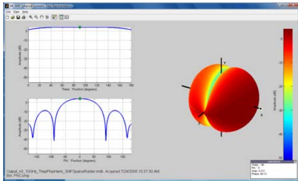
Figure 13 - Center Element of Array After IsoFilter TM
