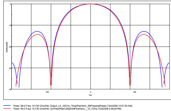
Figure 15 – Center-Element Far Field After IsoFilter TM vs. Actual Far Field of Ideal Element
