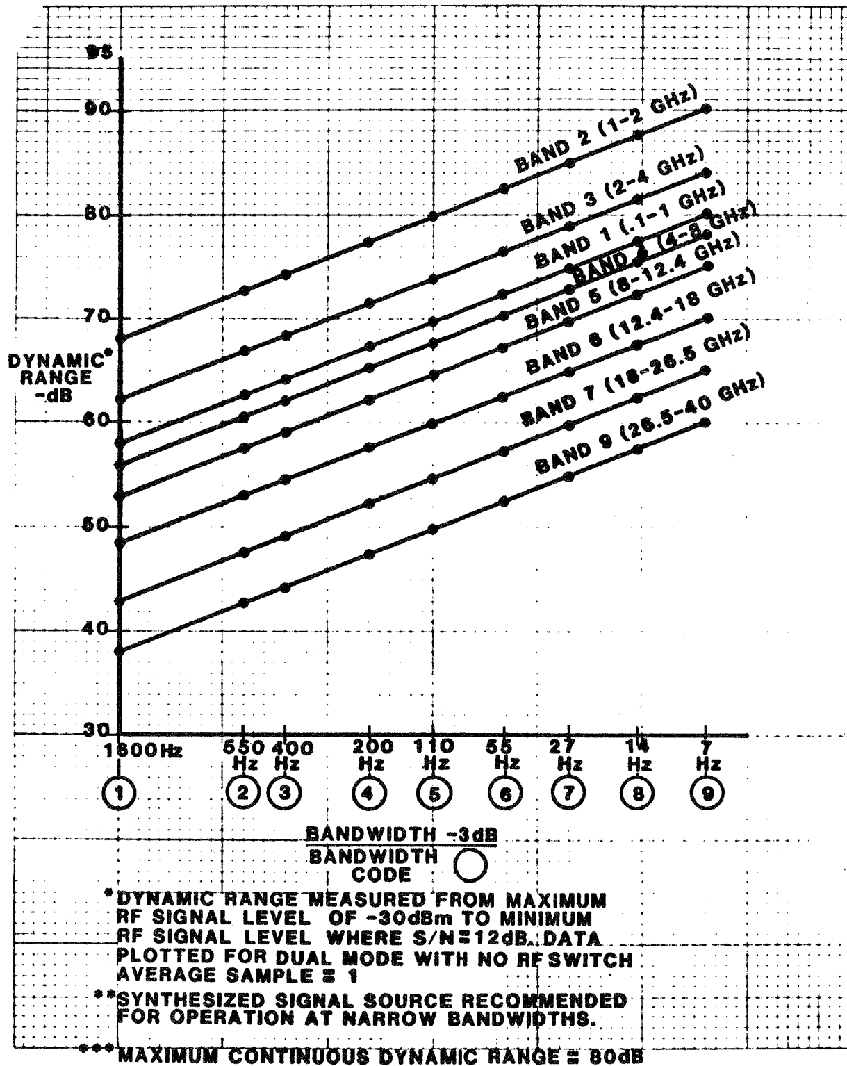
Figure 7. Signal Channel Operating Dynamic Range vs Predetection Bandwidth Selection
