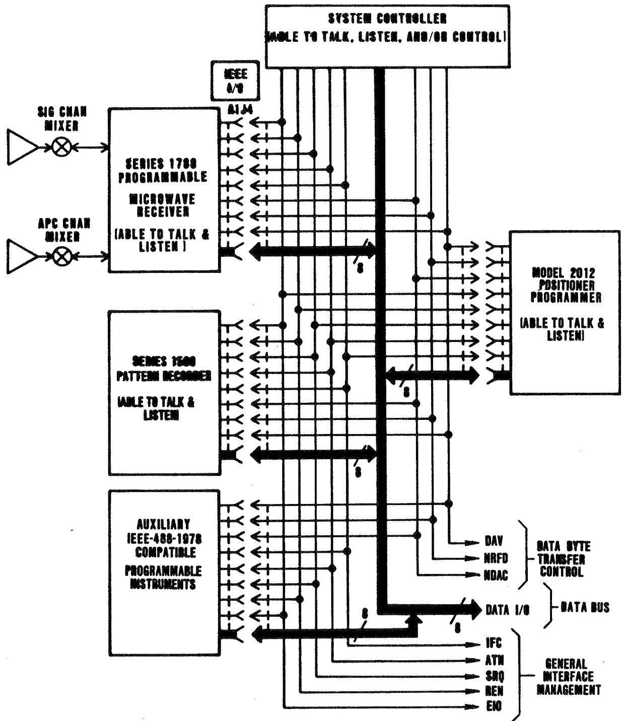
Figure 6. Series 1780 Programmable Microwave Receiver Connected to the IEEE-488-1978 Standard Data Bus
