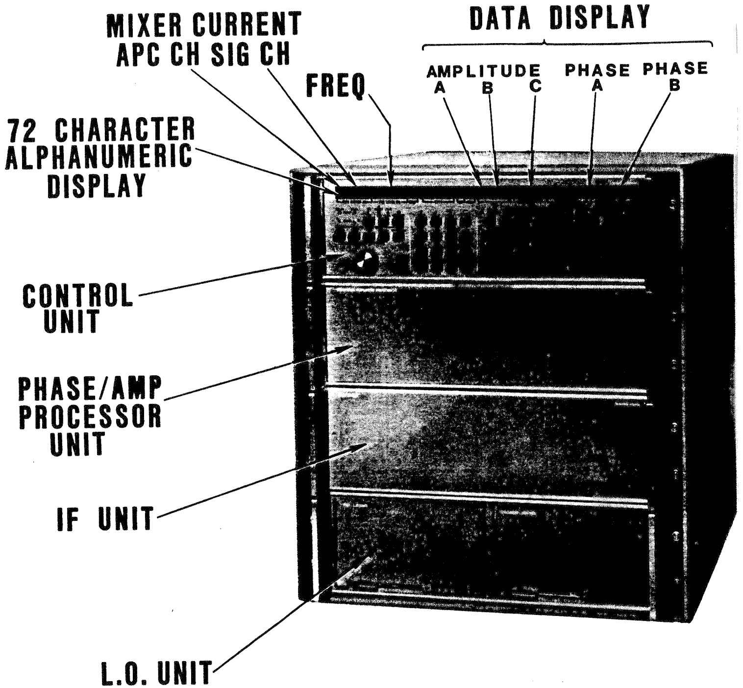
Figure 2. MODEL 1783 PROGRAMMABLE MICROWAVE RECEIVER
