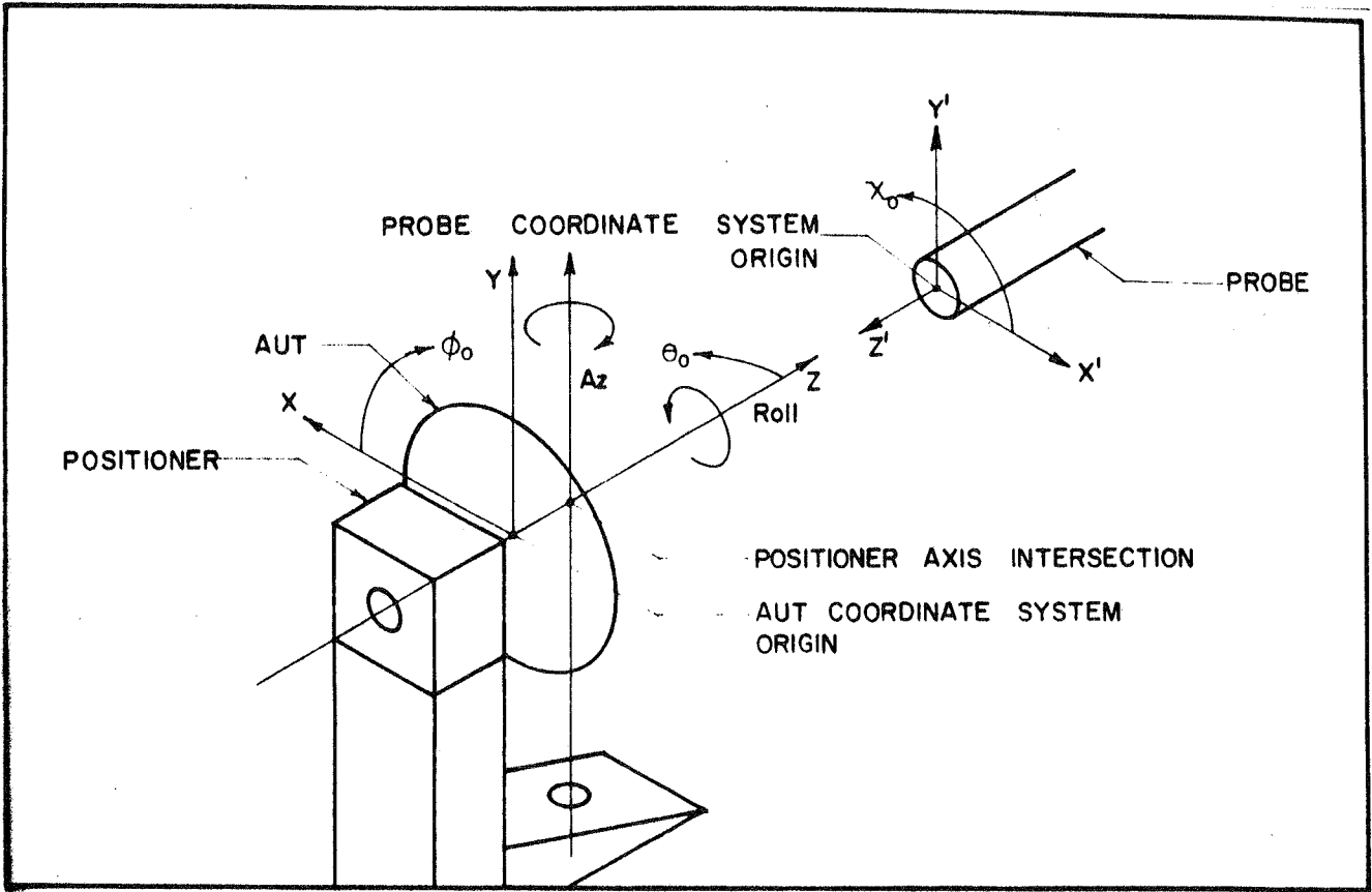
Figure 1. Coordinate Systems for Spherical Near-Field Scanning
