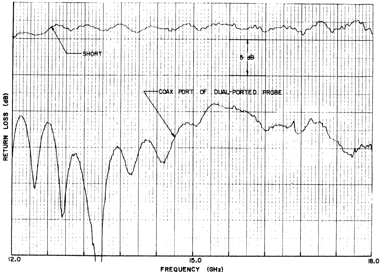
Figure 4. Return Loss on Coax Port of Dual-Polarized Spherical Near-Field Probe
