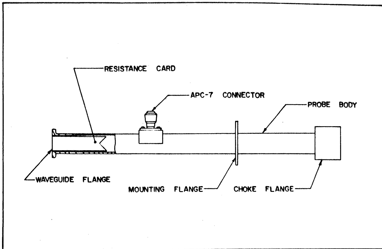
Figure 2. Dual-Polarized Spherical Near-Field Probe
