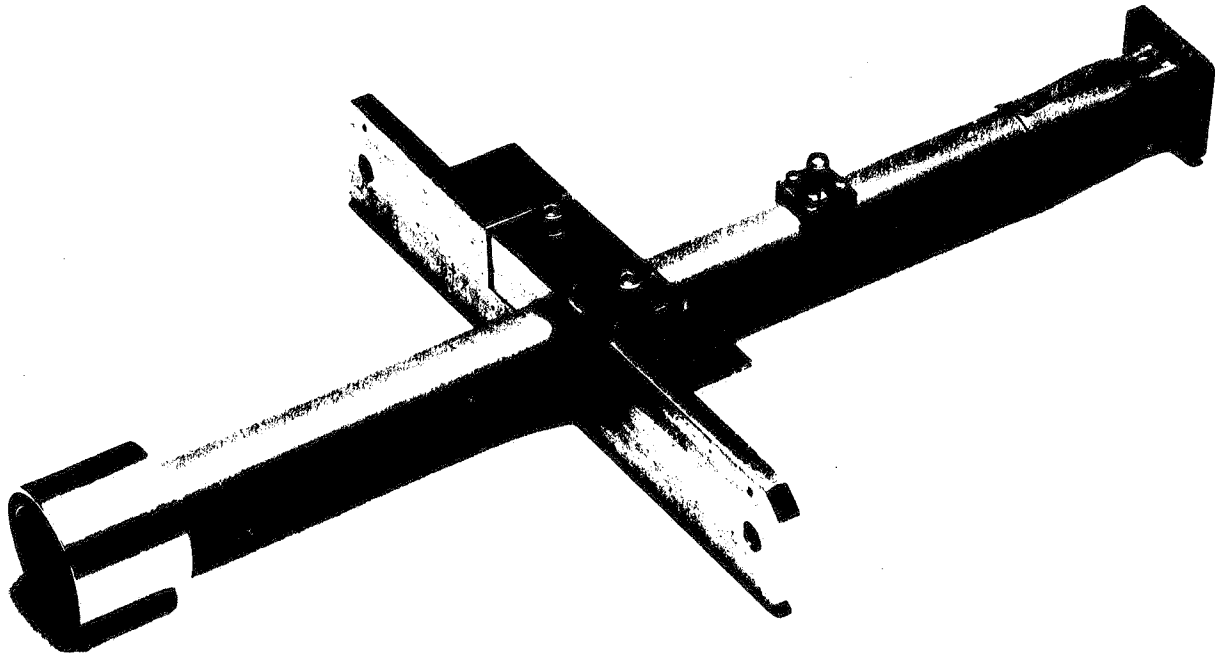
Figure 3. Electroformed prototype of dual-polarized spherical near field probe.
