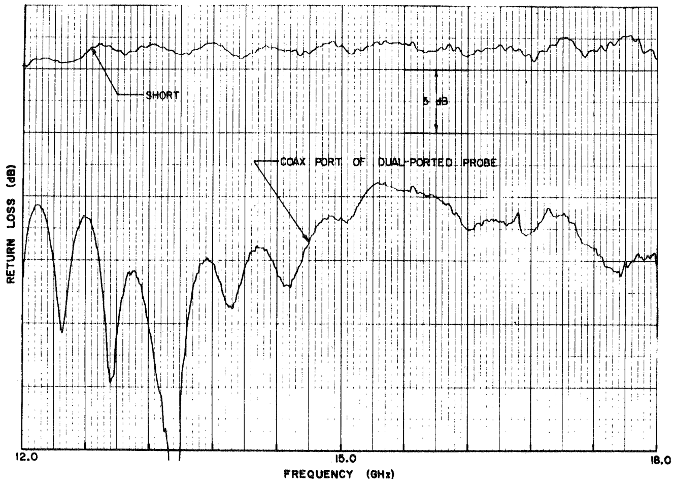
Figure 4. Return Loss on Coax Port of Dual-Polarized Spherical Near-Field Probe
