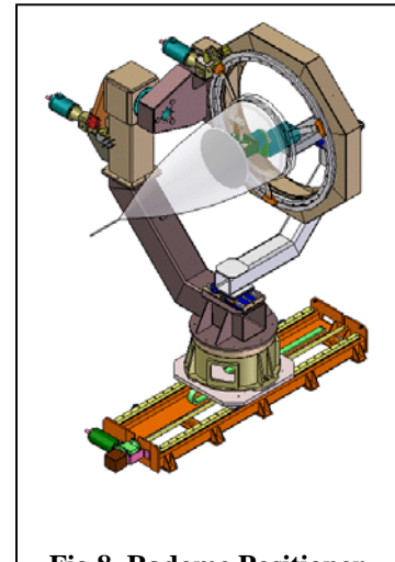
Fig.8, Radome Positioner with Antenna Mount and Auxiliary Floor Slide
