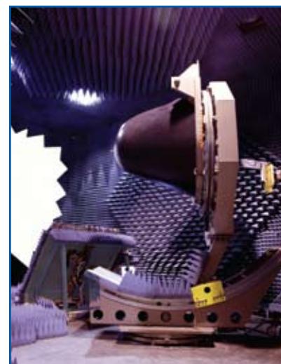
Figure 2: Radome testing in compact range system
