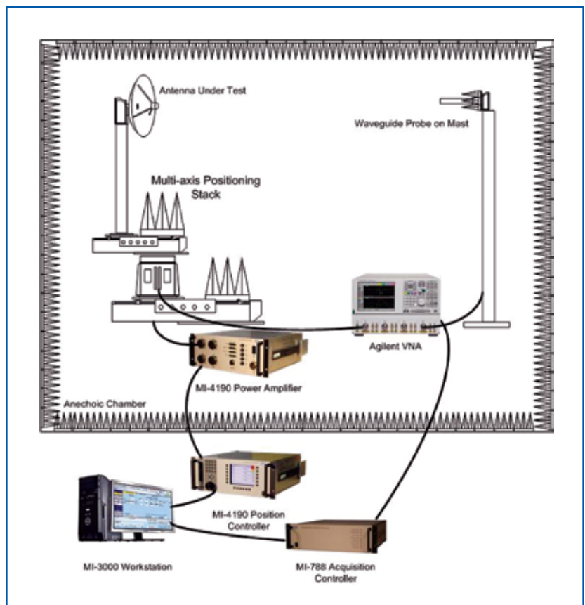
Figure 4: Antenna test system with VNA and MI-788 Networked Acquisition Controller
