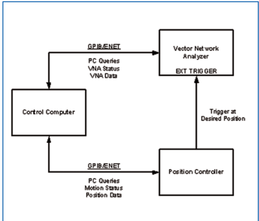
Figure 3: Simple VNA based measurement system
