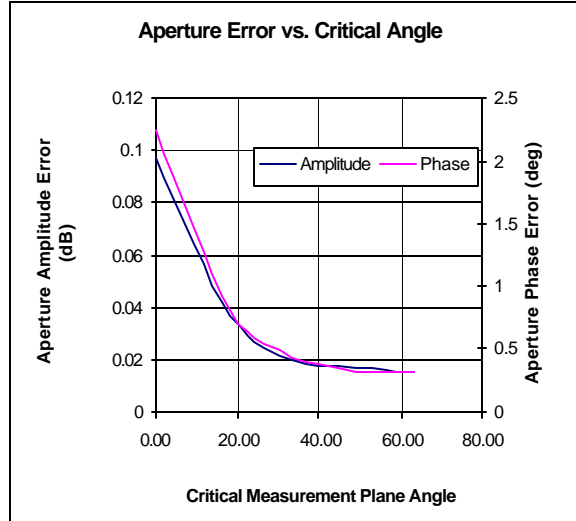
Figure 1. Accuracy of Aperture Amplitude and Phase vs. Critical Measurement Plane Angle
