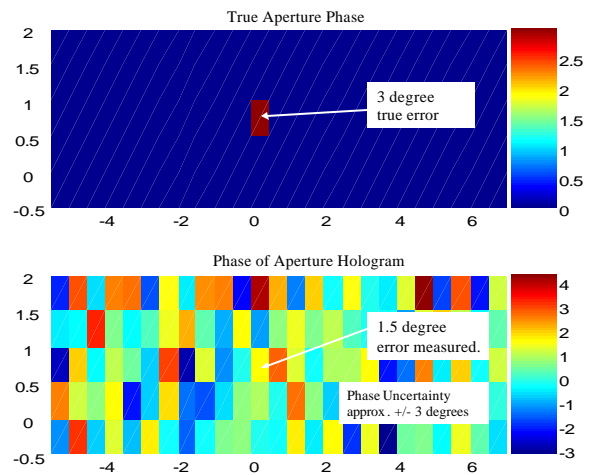
Figure 6D. True Element Phase Error Compared to Hologram Element Phase after 3rd Iteration
