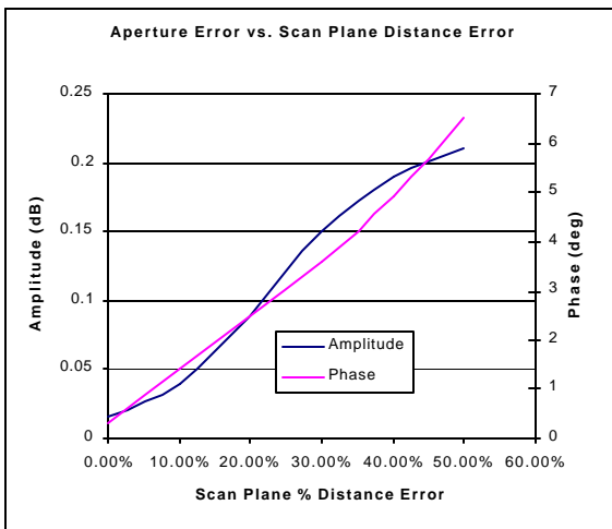
Figure 4. Accuracy of Aperture Hologram vs. Measurement Plane Distance Error
