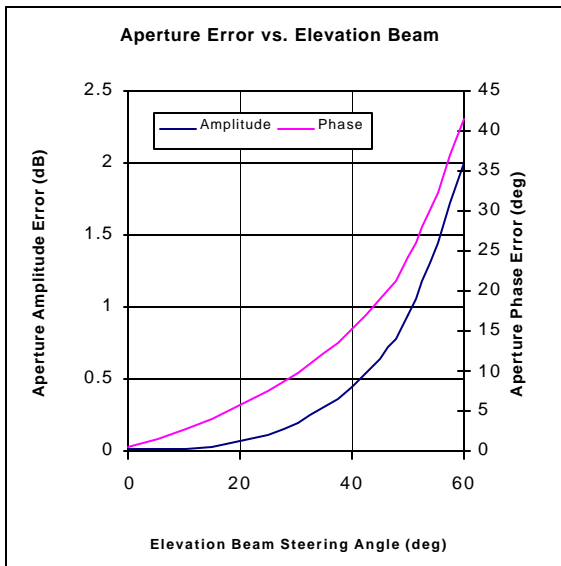
Figure 5B. Accuracy of Aperture Hologram vs. Elevation Beam Steering Angle
