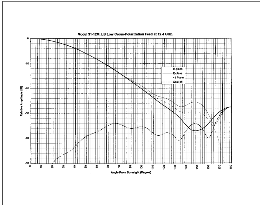
Figure 3: E-plane, H-plane, and intercardinal plane primary polarization, and intercardinal plane cross-polarization for the Model 31-12M_LB at 12.4 GHz.
