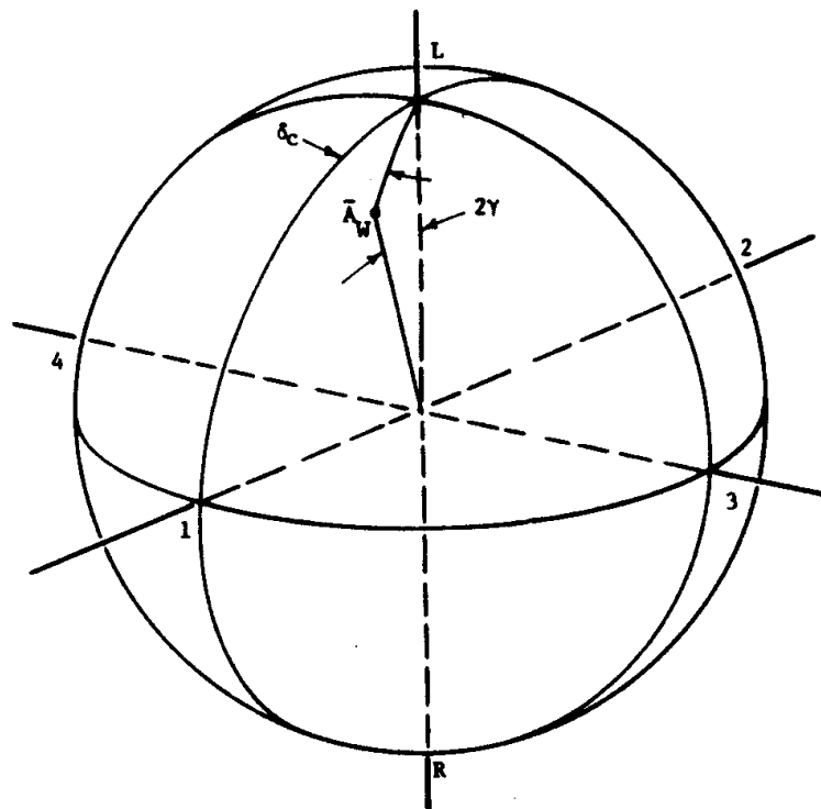
Figure 1. Poincaré sphere with polar angle 2\gamma and longitude \delta_c shown. Each point on the sphere represents a particular polarization state of a wave.
