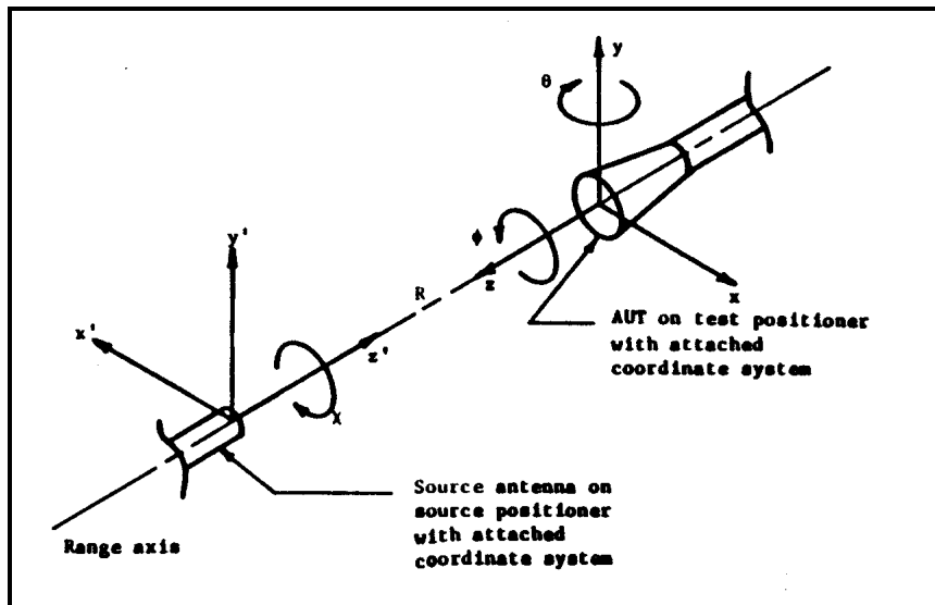
Figure 2. Coordinate system for polarization measurement.
